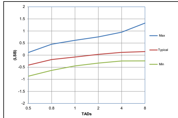
FIGURE 38-64: ADC 10-bit Mode, Single-Ended Gain Error, V_{DD} = 3.0V , V_{REF} = 3.0V , -40°C to 85°C.
