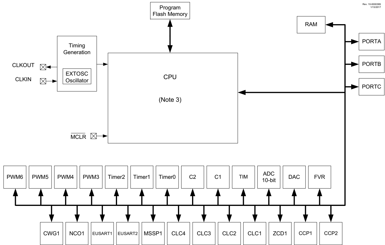
FIGURE 1-2: PIC16(L)F15344 BLOCK DIAGRAM
