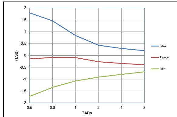
FIGURE 38-65: ADC 10-bit Mode, Single-Ended Offset Error, V_{DD} = 3.0V , V_{REF} = 3.0V , -40°C to 85°C.
