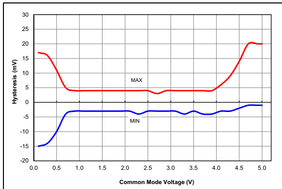
FIGURE 38-81: Comparator Offset, NP Mode (CxSP = 1), VDD = 5.5V, Typical Measured Values at 25°C.
